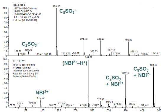
Figure 2. Top: Negative-mode ESI-MS spectrum of 9.3 \mu\text{M} \text{C}_2\text{SO}_3^- (ethansulfonate) + 11 \mu\text{M} \text{C}_8\text{SO}_3^- (octanesulfonate) + 10 \mu\text{M} \text{NBI}^{2+} ; Bottom: Positive-ion mode PIESI-MS spectrum of same solution.
