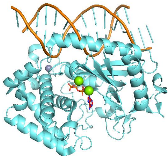
Figure 1: Crystal structure of human cGAS-DNA complex with ATP. PDB entry: 6CTA (Zhou, et al. , 2018).
